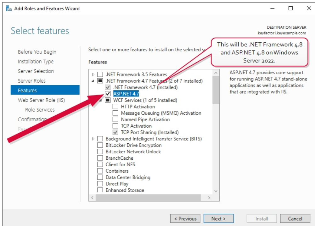
Figure 58: .NET 4.7 Feature
