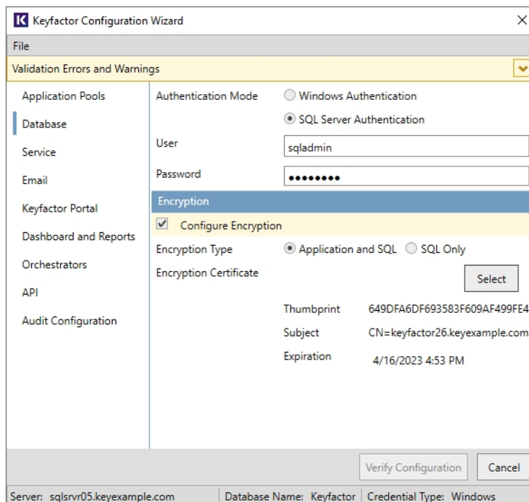
Figure 29: Configure: Database
