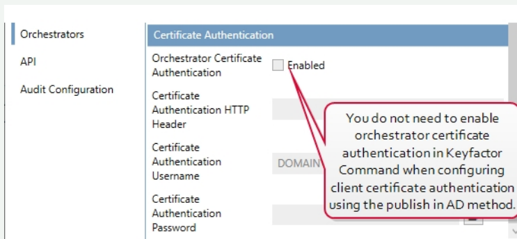
Figure 40: Client Certificate Authentication with AD Storage Does Not Require Certificate Authentication Configuration in Keyfactor Command
