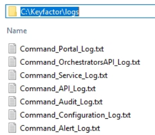
Figure 422: C:\Keyfactor\logs logs
